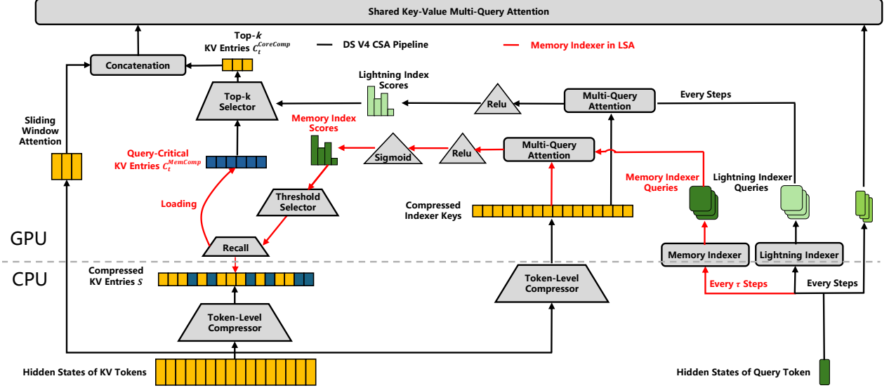
Figure 2 Architectural overview of LSA vs. CSA. The black lines denote the standard, step-by-step CSA pipelines. The red lines highlight our proposed LSA mechanism, which decouples the GPU memory footprint by leveraging a Memory Indexer to fetch historical KV chunks dynamically every \tau steps.
